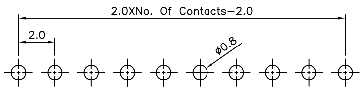
Recommended P.C.Board Layout(Top View) (PCB Board Tolerance±0.05)
