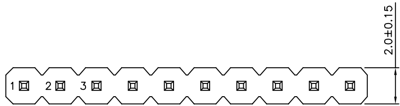
Recommended P.C.Board Layout(Top View) (PCB Board Tolerance±0.05)
